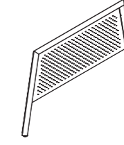
Diamond leg with modesty 40x40x1.2 mm
